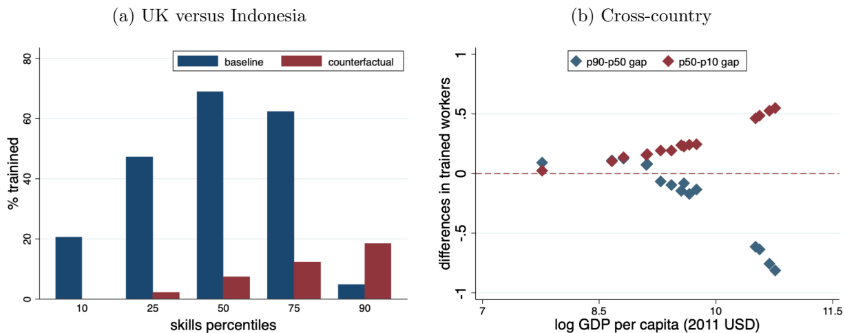
Figure 18: Training
