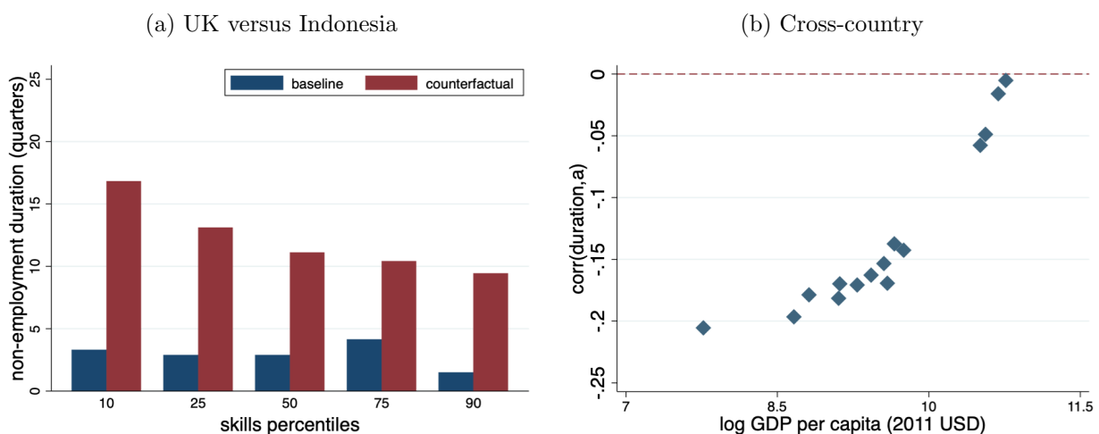
Figure 16: Non-employment duration
