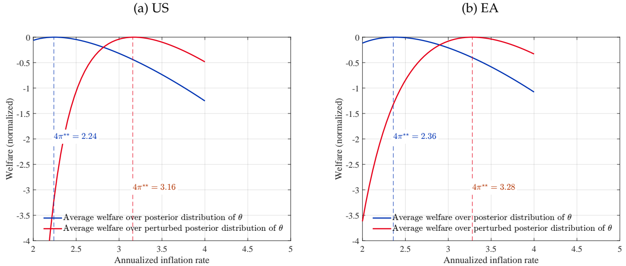
Figure 10: \mathbb{E}_\theta(\mathcal{W}(\pi, \theta))
