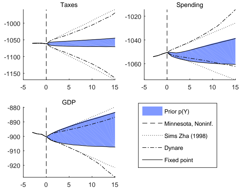
Figure 3 – Density of Taxes, Spending and GDP implied by alternative priors. Quantiles 0.05 and 0.95 of the distribution in periods 1-15 of the estimation sample.
