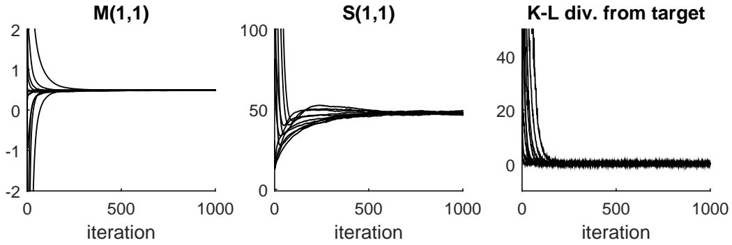
Figure 4 – Two parameters of g^z along the iterations and the estimated Kullback-Leibler divergence between p(Y) and \int_{\Theta} p(Y|\theta) g^z(\theta) d\theta along the iterations.
