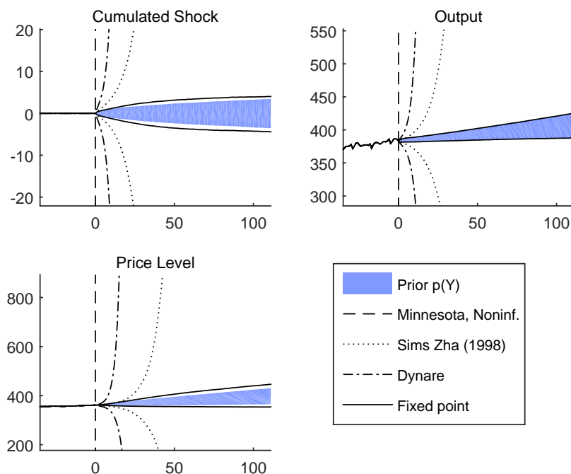
Figure 8 – Density of the observables implied by alternative priors. Quantiles 0.16 and 0.84 of the distribution in periods 1 to 111 of the estimation sample.
