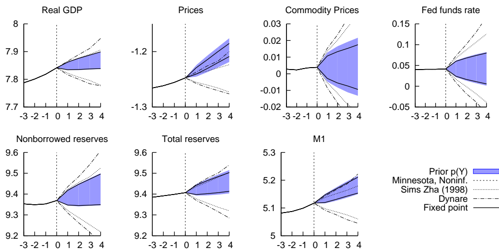
Figure 6 – Density of the observables implied by alternative priors. Quantiles 0.05 and 0.95 of the distribution in periods 1 to 4 of the estimation sample.
