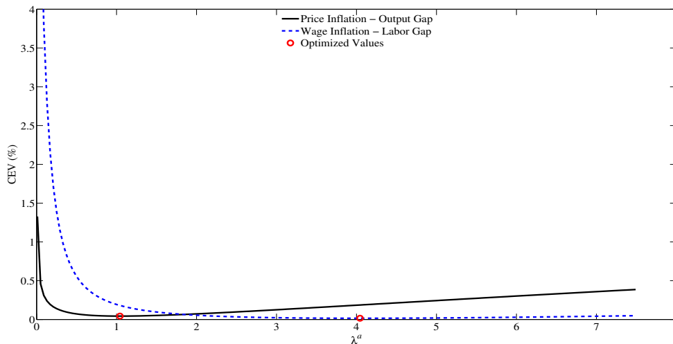
Figure 5: CEV (in percentage points) as Function of \lambda^a for Alternative Simple Mandates.
