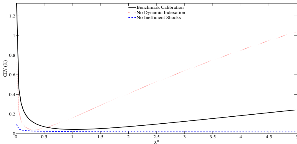
Figure 3: CEV (in percentage points) as Function of \lambda^a for Alternative Calibrations.
