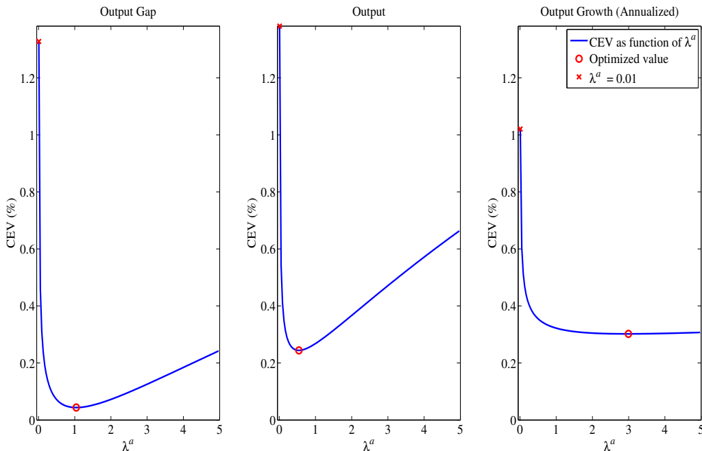
Figure 1: Consumption Equivalent Variation (percentage points) as Function of the Weight ( \lambda^a ) on Economic Activity.
