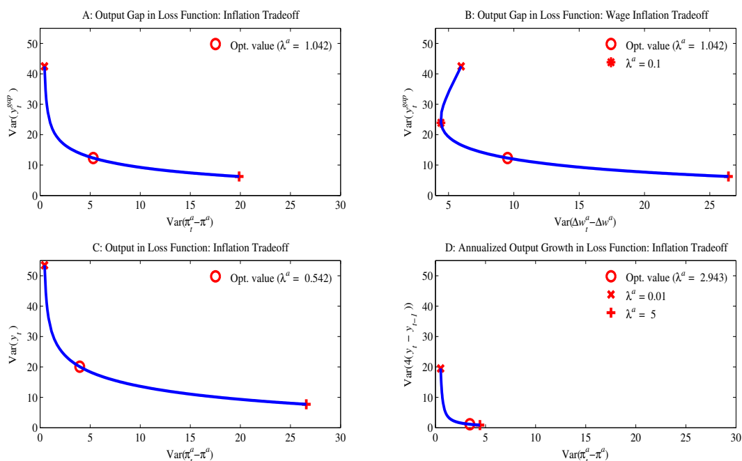
Figure 2: Variance Frontier for Alternative Resource Utilization Measures.
