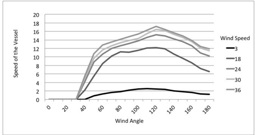
Figure 2: Polar diagram of a Clipper in 1860
