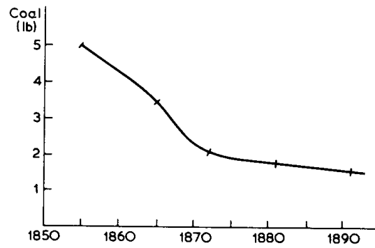
Figure 6: Coal consumption per horsepower per hour (source: Graham (1956)).
