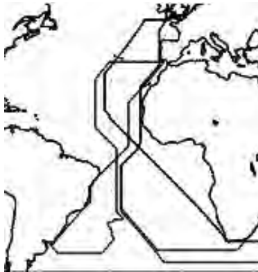
Figure 7: Optimal routes for sailing ships (month=jan; technology=clipper)
