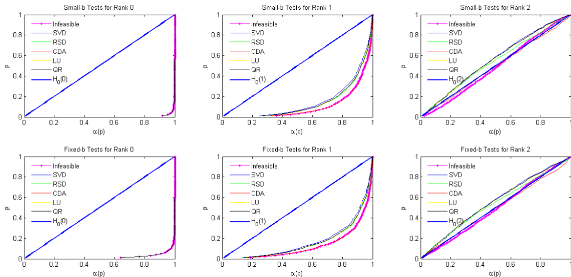
Figure 9: PP Plots for the t tests of Example 17
