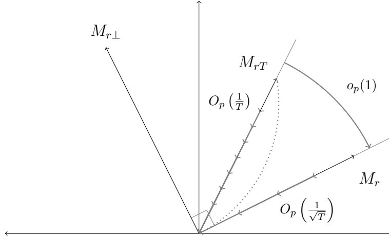
Figure 4: Convergence of a Column of \widehat{B} in Example 13.
