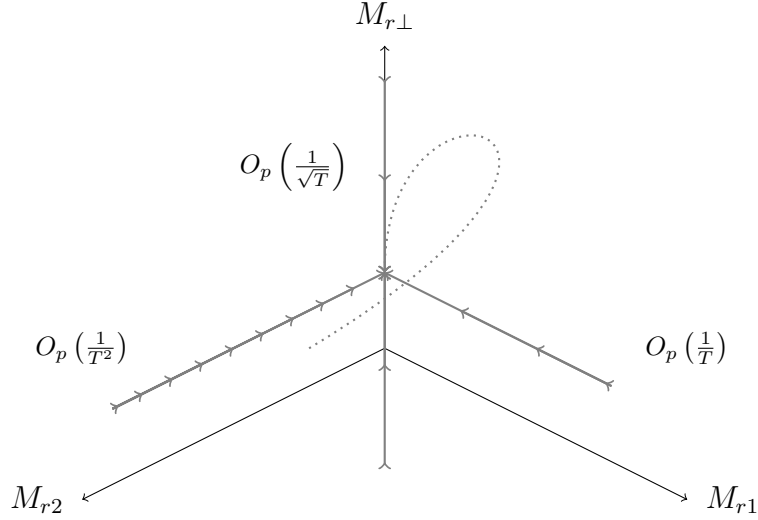
Figure 3: Convergence of a Column of \widehat{B} in Example 12.
