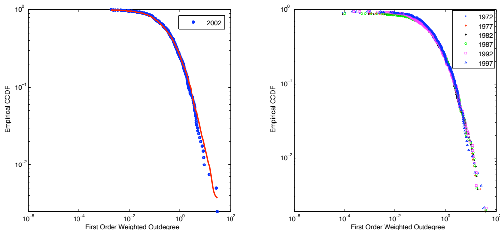
Figure 8: Empirical counter-cumulative distribution function of first-order degrees
