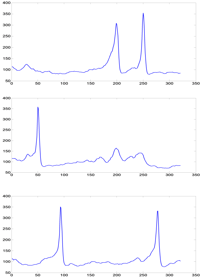
Figure 3: Simulated PD ratio, estimated model from Table 3 ( \gamma = 5 )
