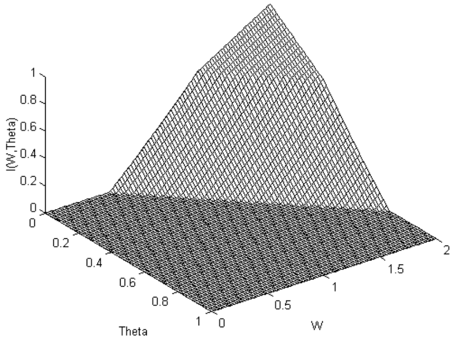
Figure 4: IMP_{w\theta} : uniform distribution, a = 0 and z = .2
