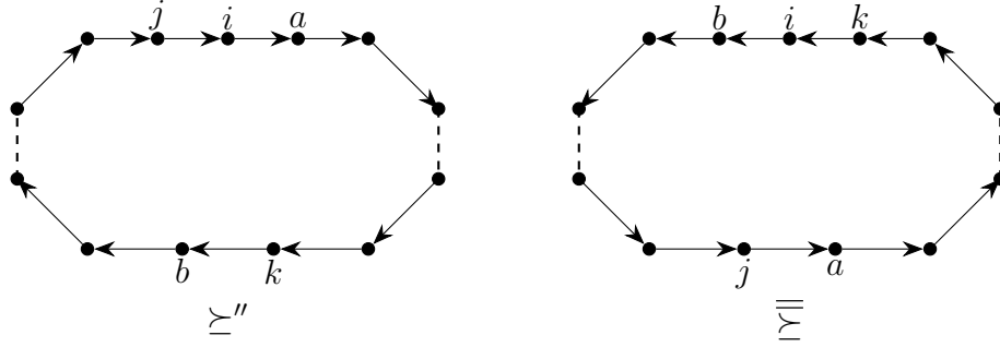
Figure 11: The set of vertices Z and all edges between vertices in Z at \Gamma(\succeq'') and \Gamma(\preceq'') .
