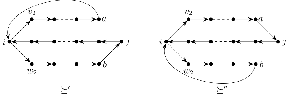
Figure 13: The set of vertices Z and all edges between vertices in Z at \Gamma(\succeq') and \Gamma(\succeq'') .
