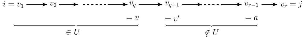
Figure 14: Path (v_1 = i, v_2, \dots, v_{r-1} = a, v_r = j) in \Gamma(\succeq) .
