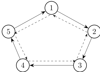
Figure 5: Friendship graph in Example 8. The continuous edges point to the best friends, while the discontinuous edges point to the second-best friends.
